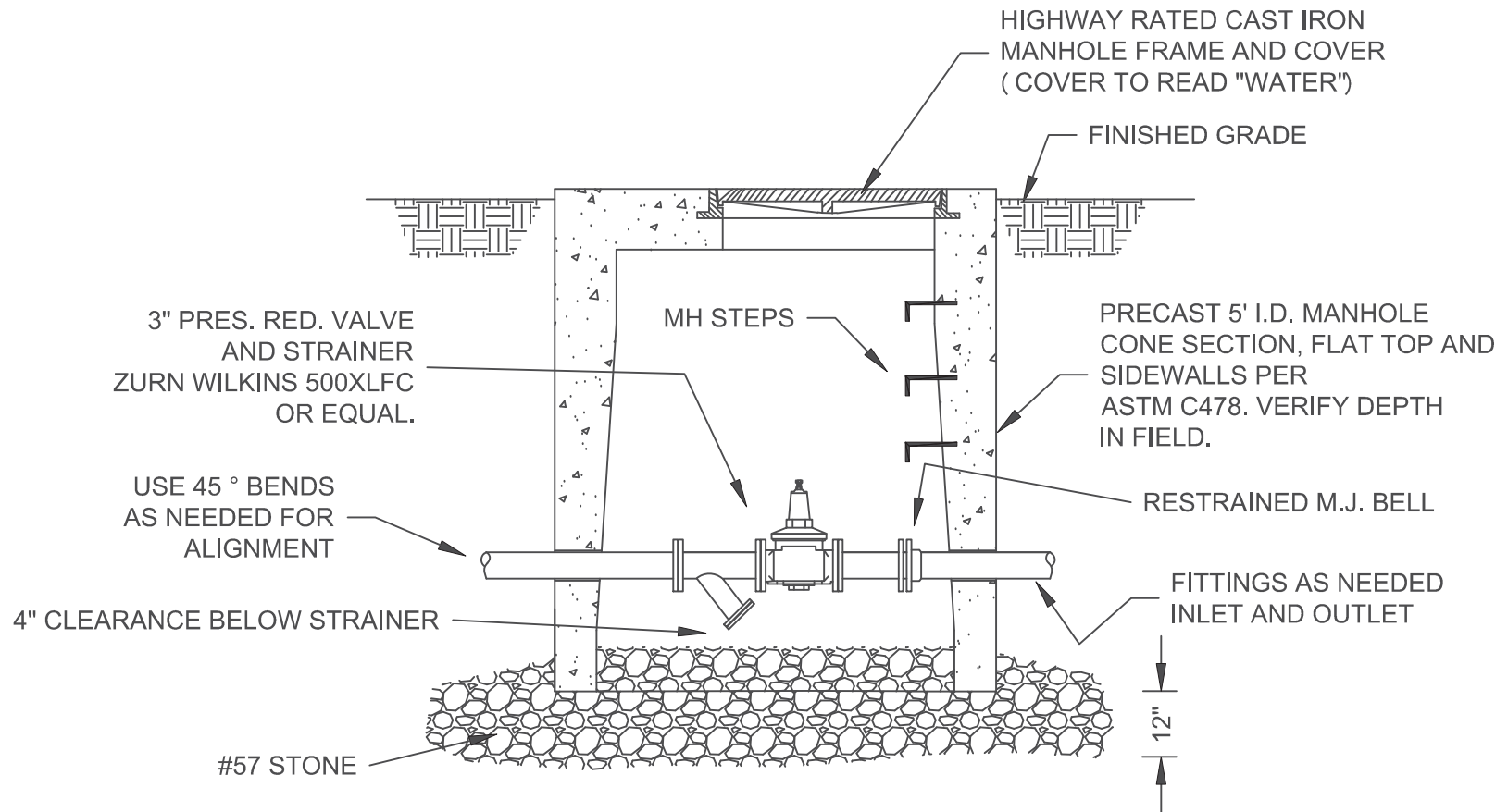
PRESSURE REDUCING VALVE DETAIL NOT TO SCALE
